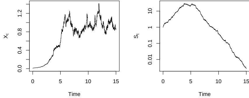
Figure 12.2 Left panel: A realization of logistic growth; compare equation (12.5). Right panel: The sensitivity S_t - note the log scale.
