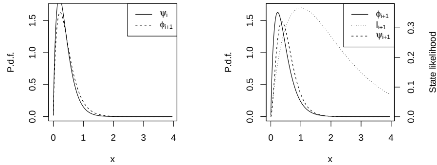
Figure 10.4 The time update (left panel) and the data update (right panel) for the Cox-Ingersoll-Ross process, illustrated for a single time step where the estimated state is low but a positive measurement Y_i = 1 arrives.
