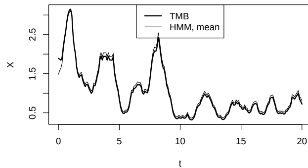
Figure 10.9 Comparison of state estimates with Template Model Builder (thick solid line) and the Hidden Markov Model method (thin solid line). For the HMM method, we show the mean in the smoothed distribution.
