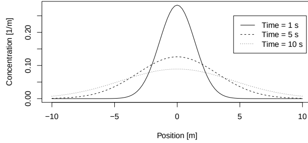
Figure 2.3 Diffusive spread. The concentration field at times t = 1, 5, 10 s with diffusivity D = 1 \text{ m}^2/\text{s} and a unit amount of material, which initially is located at the point x = 0 \text{ m} .
