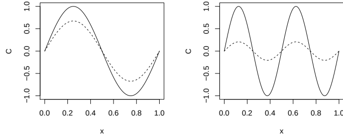
Figure 2.5 Attenuation of spatial waves by diffusion. Here the diffusivity is D = 1 and the terminal time is T = 0.01 . Solid lines: At time 0, the amplitude is 1. Dashed lines: At time T , the wave is attenuated – how much depends on the wave number. Left panel: A long wave is attenuated slowly. Right panel: A shorter wave is attenuated more quickly.
