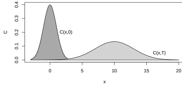
Figure 2.6 A fluid flow in one dimension which transports a substance. The plume is advected to the right with the flow; at the same time it diffuses out. The diffusivity is D = 1 , the advection is u = 2.5 , and the terminal time is T = 4 .
