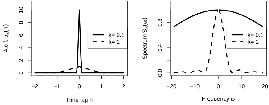
Figure 5.6 Autocorrelation function (left) and variance spectrum (right) of the difference quotient of Brownian motion.
