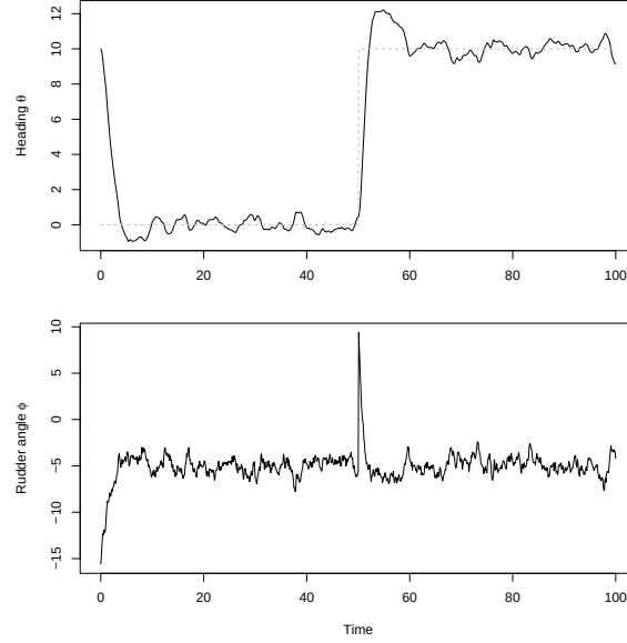
Figure 13.3 Simulation of an autopilot for a ship. The noise signal in the simulation is biased, i.e., the Brownian motion has a drift of 5. Top panel: The heading \theta_t of the ship. Included is also the desired heading \theta^{\text{REF}} (dashed), which changes during the simulation. Bottom panel: The rudder angle \phi_t , i.e., the control signal.
