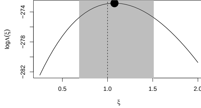
Figure 10.7 The log-likelihood \log \Lambda(\xi) of the Cox-Ingersoll-Ross model. The curve displays the log-likelihood \log \Lambda(\xi) . The vertical line indicates the “true” value used to generate the simulated data set. The point indicates the maximum, corresponding to the maximum likelihood estimate. The gray region indicates a 95 % confidence interval.
