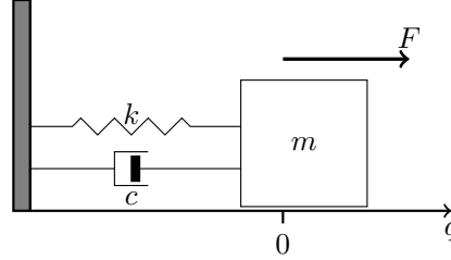
Figure 5.1 A mass-spring-damper system driven by an exogenous force is a simple example of a linear system.
