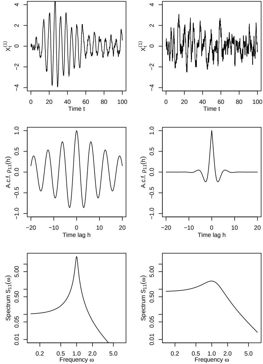
Figure 5.8 The noisy harmonic oscillator with k = 1 . Left column: \mu = 0.05 , \sigma^2 = 10 . Right column: \mu = 0.5 , \sigma^2 = 1 . Top row: Simulated sample paths of \{X_t^{(1)}\} . Middle row: The a.c.f. of \{X_t^{(1)}\} . Bottom row: The variance spectrum of \{X_t^{(1)}\} .
