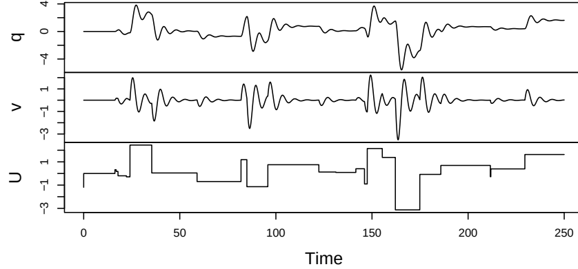
Figure 5.3 The response of the mass-spring-damper system to a force with random steps. Parameters as in Figure 5.2; \tau = 15 s. Top panel: Position Q [m]. Middle panel: Velocity V [m/s]. Bottom panel: Force U [N].
