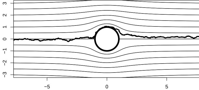
Figure 1.2 A small particle embedded in the two-dimensional flow around a cylinder. The thin lines are streamlines , i.e., the paths a water molecule follows, neglecting diffusion. The thick black line is a simulated random trajectory of a particle, which is transported with the flow, but at the same time subjected to molecular diffusion.
