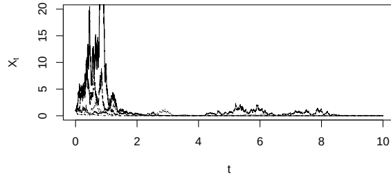
Figure 12.7 5 sample paths of Geometric Brownian Motion starting at X_0 = 1 . The parameters are r = 1 and \sigma = 2 , for which the system is stochastically stable but unstable in mean and in mean square.
