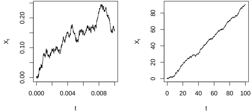
Figure 6.1 Simulation of Brownian motion with drift with u = \sigma = 1 . Left panel: t \in [0, 0.01] . Right panel: t \in [0, 100] .
