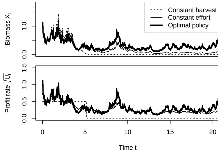
Figure 13.4 Simulation of the fisheries management system with \sigma^2 = 1/2 and three management regimes: Constant catch U_t = 1/4 until collapse, constant effort U_t = X_t/2 , and the optimal policy U_t = X_t^2 . The three simulations are done with the same realization of Brownian motion.
