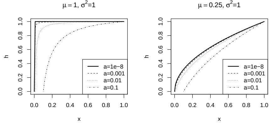
Figure 11.3 The probability of exit to the right of (a, 1) for the squared Bessel process (11.6), as function of the initial condition x , for b = 1 and different values of a . Left panel: With \mu = 1 , \sigma^2 = 1 , the probability approaches 1 as a \rightarrow 0 . Right panel: With \mu = 0.25 , \sigma^2 = 1 , the probability of exit to the right approaches \sqrt{x} as a \rightarrow 0 .
