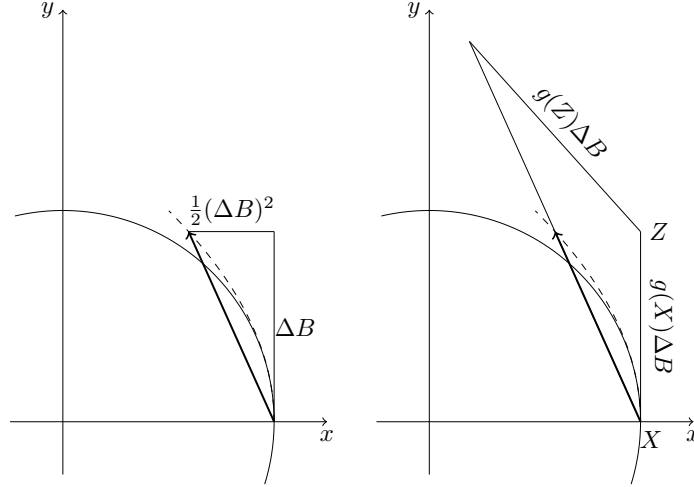
Figure 8.4 The Mil'shtein scheme (left) and the Heun scheme (right) for Brownian motion on the unit circle. One step is shown, starting at position (X_t, Y_t) = (1, 0) . Note that the schemes return a point on the supporting parabola (dashed).
