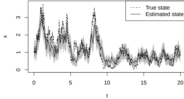
Figure 10.5 Estimated (solid) and true (dashed) state trajectory for the Cox-Ingersoll-Ross process. The estimate is the mean in the estimated distribution \psi_i . Included is also 67 % confidence intervals, derived from the estimated distribution \psi_i .
