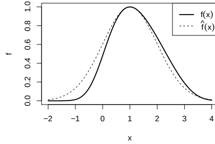
Figure 10.8 The function f(x) and its approximation \hat{f}(x) .
