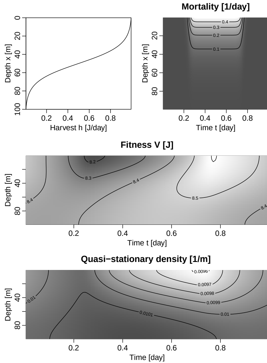
Figure 11.5 Diel vertical migration of zooplankton. Top left: The energy harvest h(x) plotted against depth. Top right: Mortality \mu(x, t) as a function of time and depth. Middle: Resulting fitness V(x, t) . Bottom: Quasi-stationary distribution \rho(x, t) .
