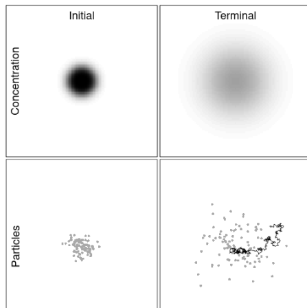
Figure 2.1 Diffusion in a container in two dimensions. Top panels: Concentration fields. Bottom panels: Position of 100 molecules. Left panels: Initially, the solute is concentrated at the center. Right panels: After some time, the solute is less concentrated. The bottom right panel also includes the trajectory of one molecule; notice its irregular appearance.
