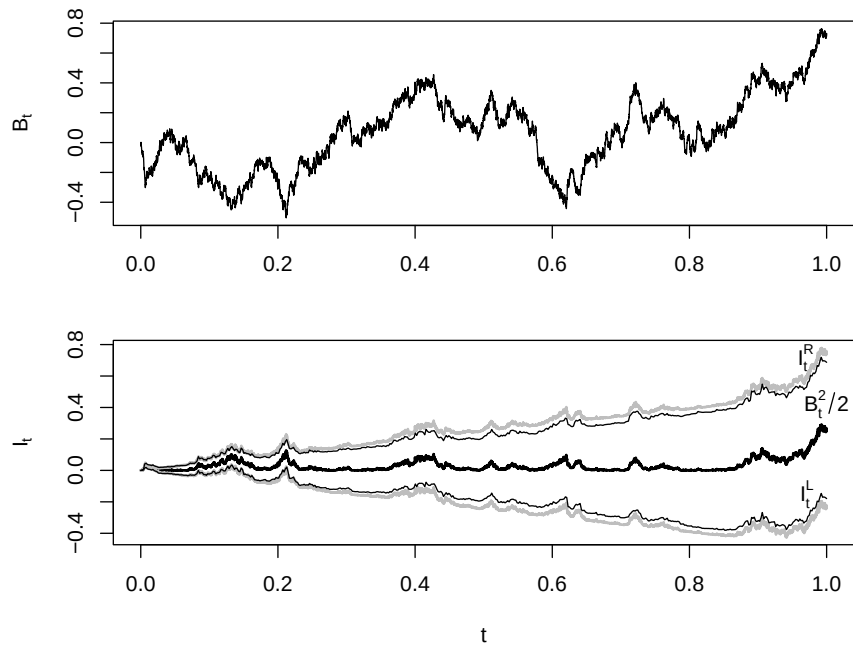
Figure 6.6 Top panel: A realization of Brownian motion B_t for t \in [0, 1] . Bottom panel: Left hand ( I_t^L ) and right hand ( I_t^R ) approximations of \int_0^t B_s dB_s . Thick grey lines use a fine grid ( h = 2^{-13} ) while thin black lines use a coarse grid ( h = 2^{-9} ). Included is also B_t^2/2 (thick solid line).
