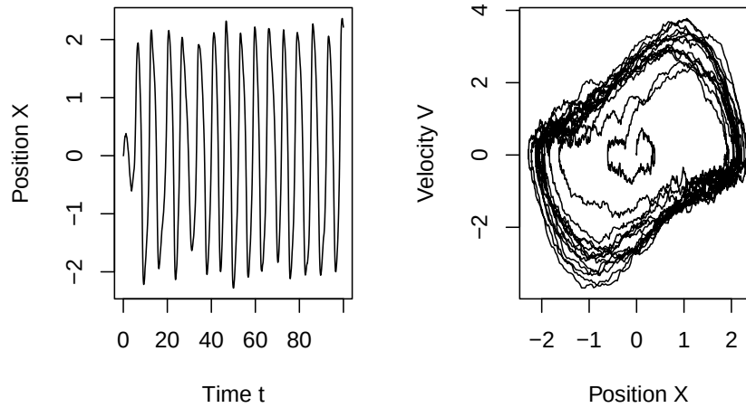
Figure 6.4 The stochastic van der Pol oscillator with \mu = 1 , \sigma = 1/2 . Left panel: The position X_t vs. time. Right panel: Trajectories in the phase plane (X_t, V_t) .
