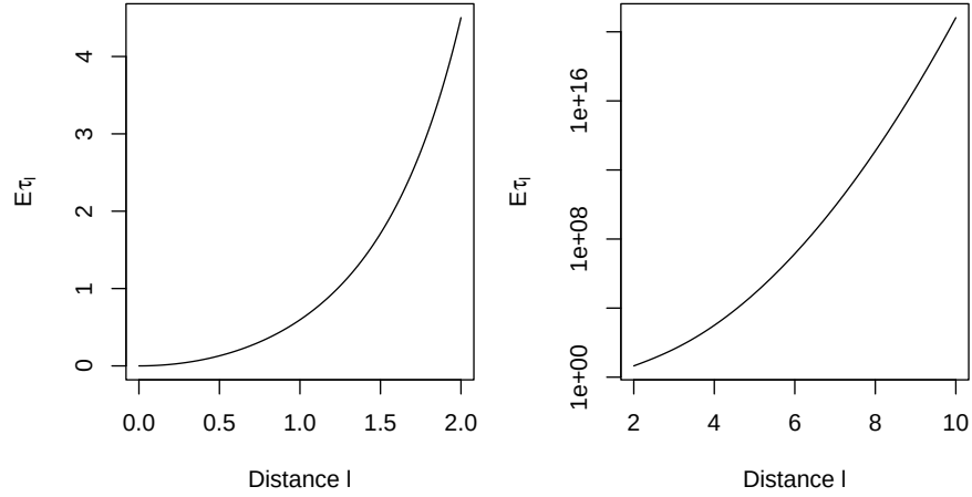
Figure 11.2 Expected time for an Ornstein-Uhlenbeck process to exit the domain [-l, l] , as a function of the domain size l . Left panel: The expected time for low values of l . Right panel: The expected time for higher values of l . Note the log scale. In this panel, the approximation (11.3) would be indistinguishable from the full expression.
