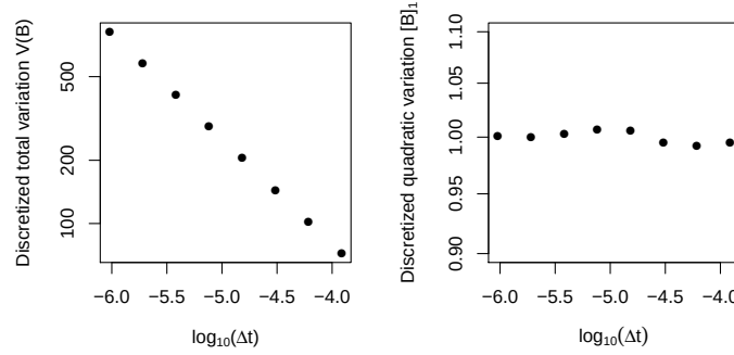
Figure 4.3 Estimating the variation (left panel) and the quadratic variation (right panel) of one sample path of Brownian motion on [0, 1] with discretization. Notice the logarithmic axis in the total variation. As the time discretization becomes finer, the total variation diverges to infinity, while the quadratic variation appears to converge to 1.
