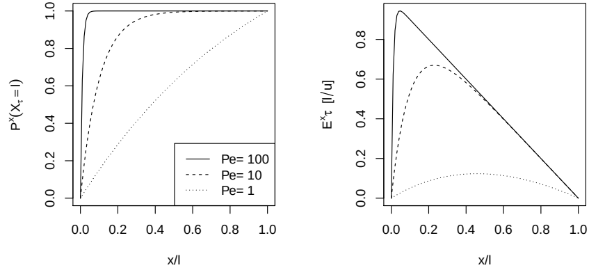
Figure 11.1 Exit behavior for Brownian motion with drift, for various Péclet numbers. Left panel: The probability of exiting to the right, as a function of the dimensionless initial position x/l . Right panel: The expected time to exit, as a function x/l , and measured in units of the advective time scale l/u .
