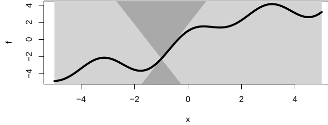
Figure 8.1 Lipschitz continuity. The function x \mapsto x + \sin x + \cos 2x is Lipschitz continuous with Lipschitz constant 4. For each point x , this restricts the graph to a cone, indicated by light gray for the point x = -1 ; the dark gray set is a “forbidden zone”.
