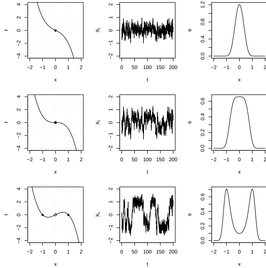
Figure 12.3 A pitchfork bifurcation in the double well model (12.8) with \sigma = 1/2 . Left panels: The drift f(x) . Stable equilibria of f are marked with solid circles and unstable equilibria are marked with open circles. Middle panels: Simulations starting at X_0 = 0 ; the same realization of Brownian motion is used in the three panels. Right panels: The stationary probability density. Upper panels: \mu = -1 . Middle panels: \mu = 0 . Lower panels: \mu = 1 .
