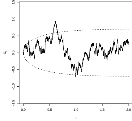
Figure 7.2 A realization of the Ornstein-Uhlenbeck process \{X_t\} given by the SDE dX_t = -\lambda X_t dt + \sigma dB_t (7.3) (solid) with X_0 = 0 , \lambda = 1 , \sigma = 1 . Included is also plus/minus the standard deviation of X_t (dashed).
