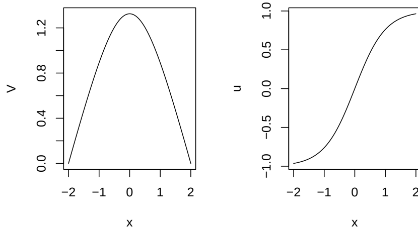
Figure 13.2 Value function (left) and optimal strategy (right) for the “swim left or right” Example 13.6.1.
