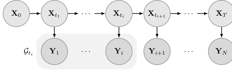
Figure 10.1 Probabilistic graphical model of the random variables in the filtering problem. The measurement equation specifies the conditional distribution of Y_i given X_{t_i} , and the stochastic differential equation specifies the conditional distribution of X_{t_{i+1}} given X_{t_i} . The shaded region contains the measurements in \mathcal{G}_{t_i} , i.e., those which are used for the state estimate \psi_i and the state prediction \phi_{i+1}
