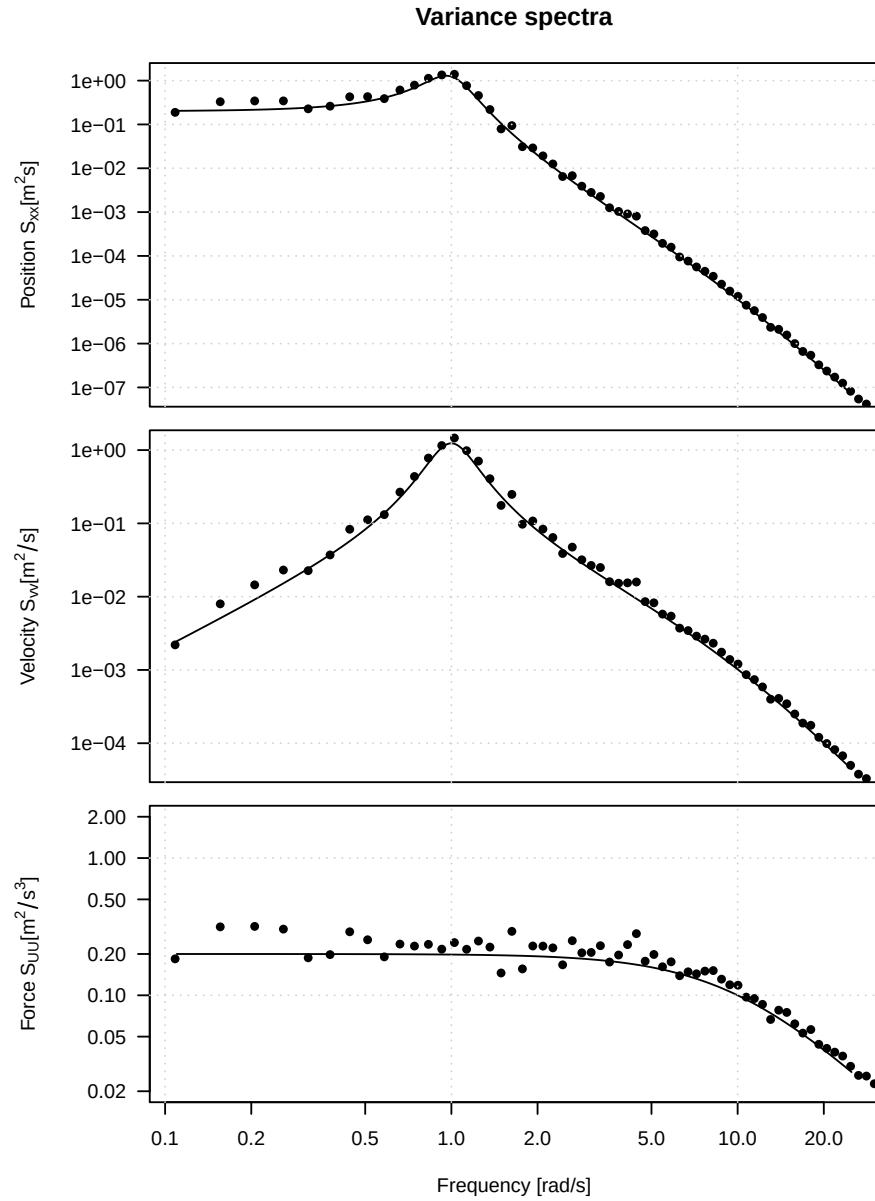
Figure 5.5 Variance spectrum of position, velocity, and force for the mass-spring-damper system. Lines are the analytical expressions. Dots are estimated spectra based on simulation of the process. The average time between jumps in the force is \tau = 0.1 s.
