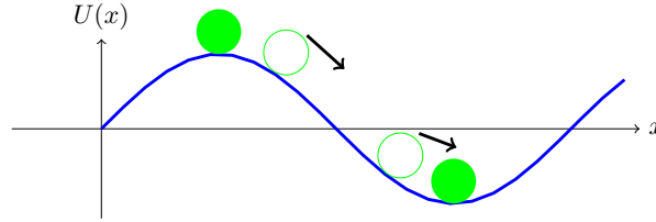
Figure 12.1 Stability for a rolling ball with friction. The hilltop forms an unstable equilibrium, while the bottom forms a stable one. Almost all solutions are stable and converge to the bottom.
