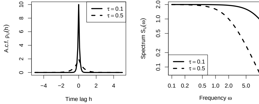
Figure 5.4 Autocovariance function and variance spectrum (in log scales) of the piecewise constant force process \{U_t : t \geq 0\} , for two values of the time constant \tau . The variance \sigma^2 is chosen so that \sigma^2\tau = 1 . Note, in the spectrum, that the cut-off frequency 1/\tau marks a transition from low-frequency behavior to high-frequency behavior.
