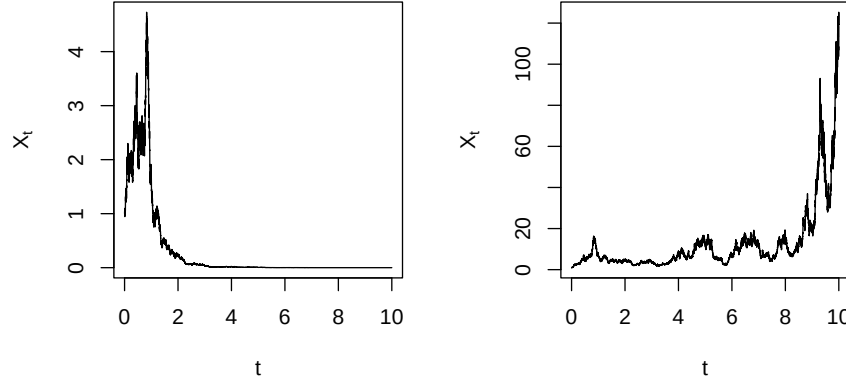
Figure 6.3 Simulation of geometric Brownian motion. Left panel: r = -0.5 , \sigma = 1 . Right panel: r = 1 , \sigma = 1 .
