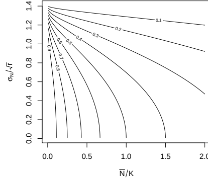
Figure 12.4 Contour plot of the non-dimensional function \eta(\frac{\bar{N}}{K}, \frac{\sigma_N}{\sqrt{r}}) which determines the expected feeding rate of a predator.
