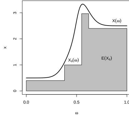
Figure 3.3 Expectation as integrals over sample space \Omega . Here, \Omega = [0, 1] . A non-negative random variable X is bounded below by a simple random variable X_s . If the probability measure is uniform, then expectation corresponds to area under the curve; e.g., \mathbf{E}X_s corresponds to the gray area.
