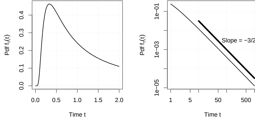
Figure 4.5 The p.d.f. of the hitting time \tau = \inf\{t : B_t = 1\} . Left panel: The initial part of the curve. Right panel: The tail of the curve. Notice the log-scales. Included is also a straight line corresponding to a power law decay \sim t^{-3/2} .
