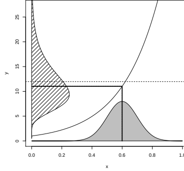
Figure 7.1 Two random variables X \sim N(0.6, 0.1) and Y = \exp 4X . The gray and shaded region displays the p.d.f. of X and Y , rescaled. Solid lines indicate medians; the dashed line indicates \mathbf{E}Y .
