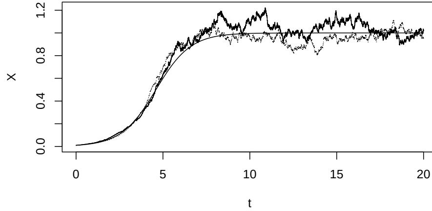
Figure 1.3 Two simulated sample paths (solid and dotted erratic curves) of the stochastic logistic growth model (1.5) with g(x) = \sigma x of a bacterial population with g(x) = \sigma x . A noise-free simulation is included (thin black line). Parameters are r = K = 1 , \sigma = 0.1 , X_0 = 0.01 . The computational time step used is 0.001.
