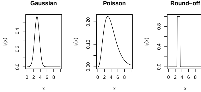
Figure 10.3 Three examples of state likelihood functions: To the left, an observation Y = 3 with Y \sim N(X, 1/2) . In the middle, an observation Y = 3 with Y \sim \text{Poisson}(X) . To the right, an observation Y = 3 with Y being X rounded to the nearest integer. Note that these are likelihood functions of the state X and not probability density functions of X .
