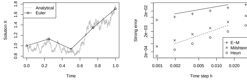
Figure 8.3 Geometric Brownian motion and its discretization. The parameters are r = 0.5 , \sigma = 0.5 , x = 1 , T = 1 . Left panel: A single sample path of the analytical solution evaluated on a very fine time grid (grey), and the Euler-Maruyama approximation with a coarse time step, h = 0.25 . Right panel: The mean absolute error of the Euler-Maruyama scheme, the Mil'shtein scheme, and the Heun scheme, plotted against the time step h . The errors are based on 100,000 realizations. Included are also straight lines corresponding to strong orders of 0.5 and 1.0.
